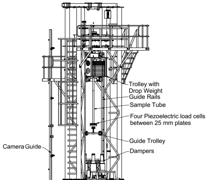
Figure 1: Overview of the layout of the DIT (Knox, et al, 2018a).
