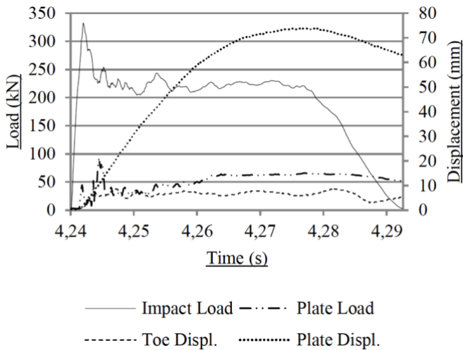
Figure 4: DIT Load and displacement as a function of time for a single impulse (Knox, et al, 2018a)
