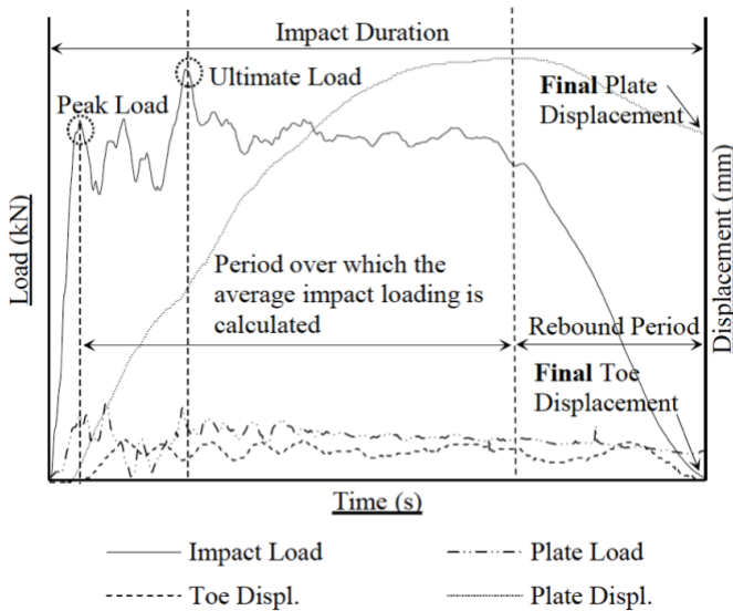
Figure 3: Illustration of the some of the data categories reported from the DIT per sample (Knox, et al, 2018a)
