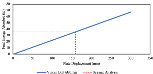
Figure 10: Back analysis of energy absorbed under pure tensile loading for a given displacement.
