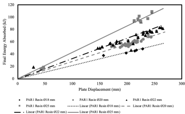
Figure 6: Summary of qualification tests on NCM's PAR1 Resin Bolts
