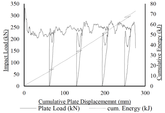
Figure 5: DIT Impact and Cumulative Energy as a function of plate displacement (Knox, et al, 2018a)
