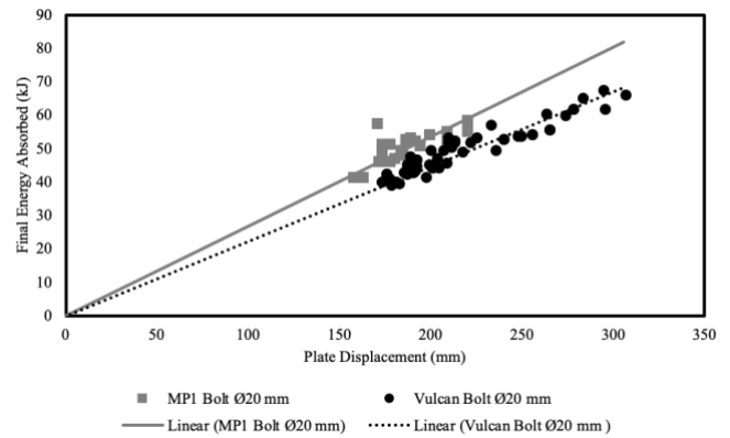
Figure 7: Summary of qualification tests on NCM's Vulcan Bolt and MPI Bolt
