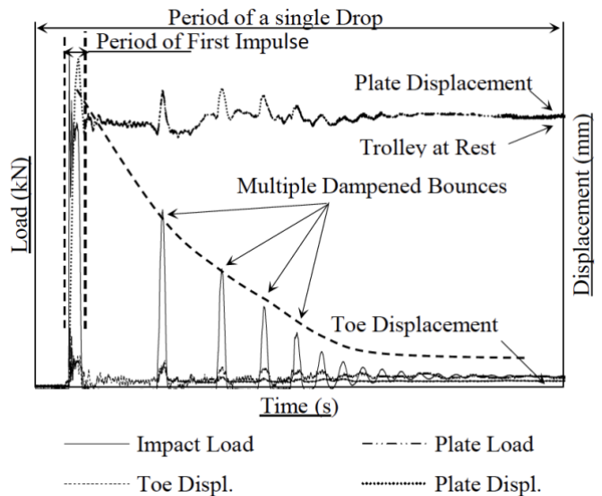
Figure 2: Typical load and displacements for a single drop on the DIT (Knox, et al, 2018a)
